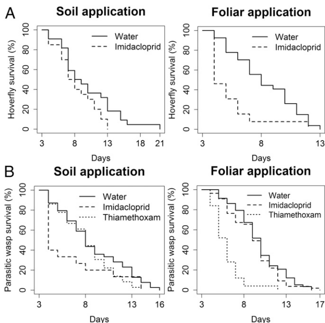
Fig. 2. Survival of beneficial insects fed on honeydew contaminated with neonicotinoid insecticides. Survival curves estimated by Kaplan–Meier of (A) the pollinating hoverfly S. rueppellii , and (B), the parasitic wasp A. pseudococci fed on honeydew of P. citri feeding on water-treated trees or on honeydew of P. citri feeding on soil- (Left) or foliar-treated trees (Right) with the neonicotinoid insecticides imidacloprid or thiamethoxam.
